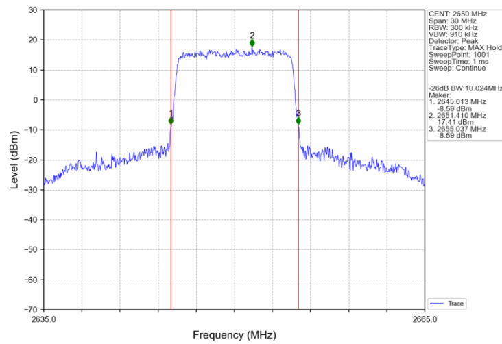
Band41 10MHz 16QAM HCH 2650MHz RB 50 0 NTNV
