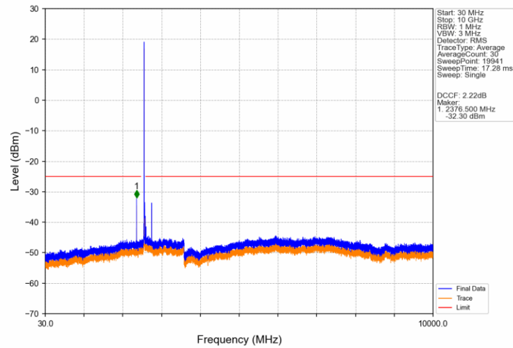
Band38 15MHz 16QAM LCH 2577.5MHz RB 1 0 NTNV
