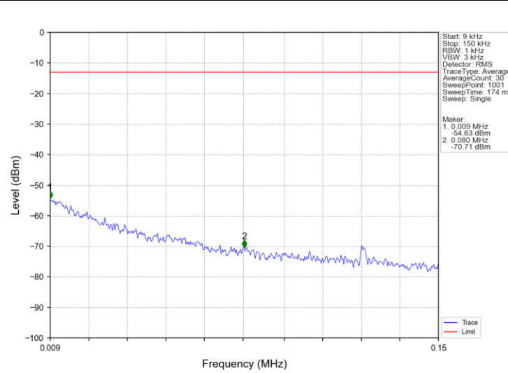
Band4 5MHz 16QAM HCH 1752.5MHz RB 1 0 NTV
