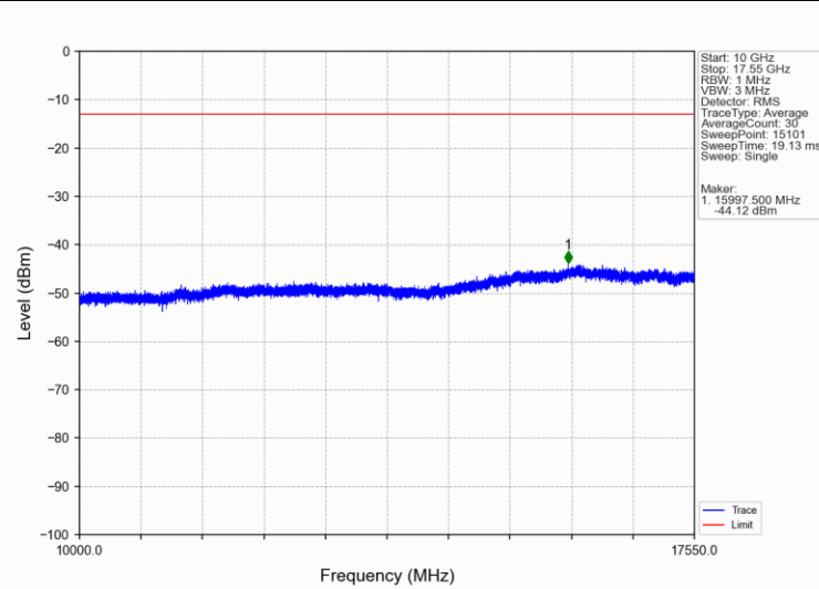
Band4 5MHz 16QAM MCH 1732.5MHz RB 1 0 NTV
