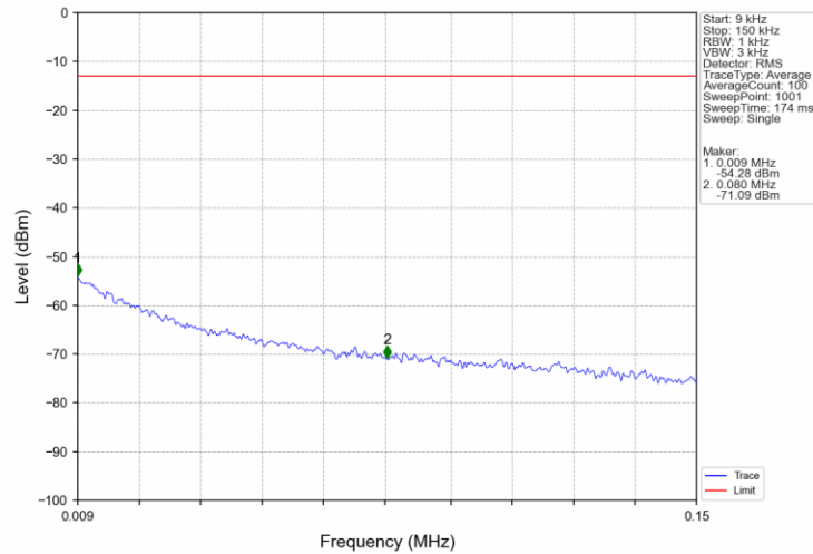
Band2_1.4MHz_QPSK_LCH_1850.7MHz_RB_1_0_NTNV
