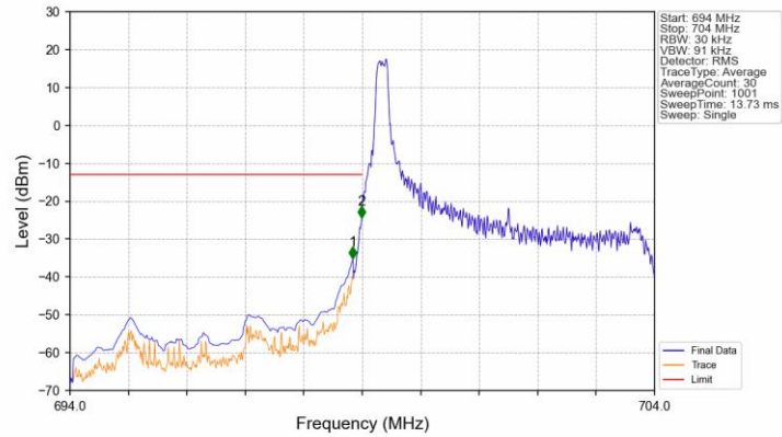
Band12_5MHz_QPSK_LCH_701.5MHz_RB_1_0_NTNV
