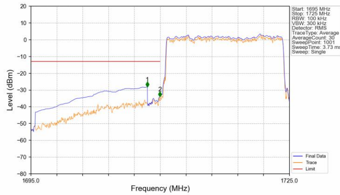
Band4_15MHz_16QAM_LCH_1717.5MHz_RB_75_0_NTNV
