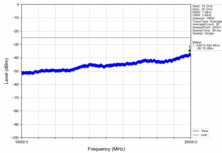
Band7_10MHz_16QAM_LCH_2505MHz_RB_1_0_NTNV
