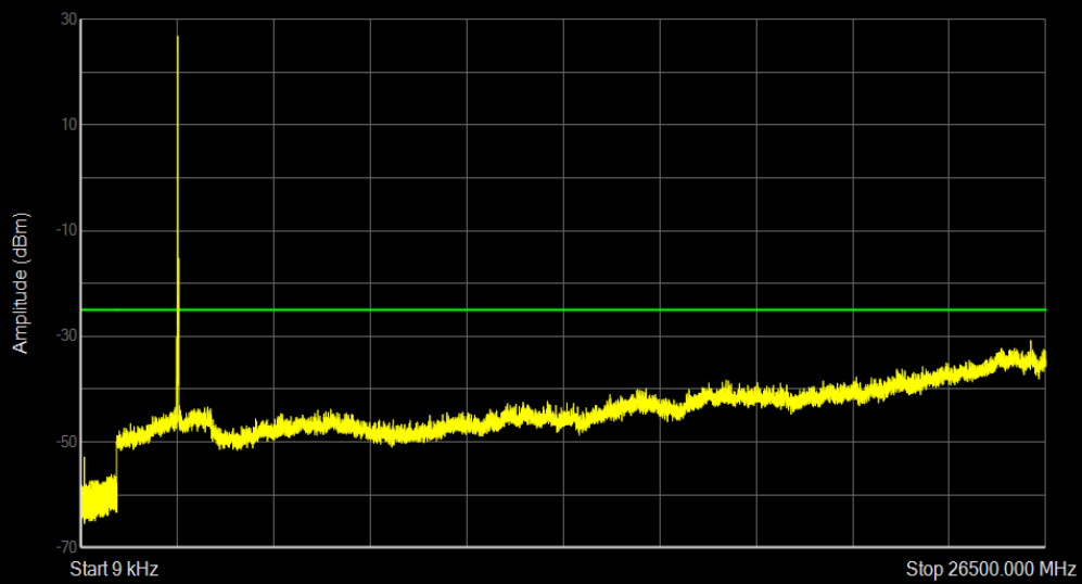
Band41 16QAM BW=15MHz Channel=41515 RB Size=1 Position=#0
