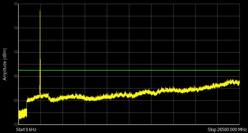
Band41 16QAM BW=20MHz Channel=40620 RB Size=1 Position=#0
