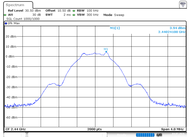
BLE_1M_Middle_Channel
