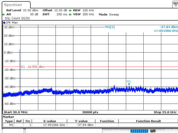
BLE_1M_Low_Channel
