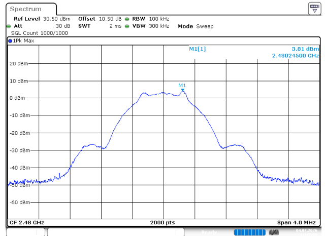
BLE_1M_High_Channel
