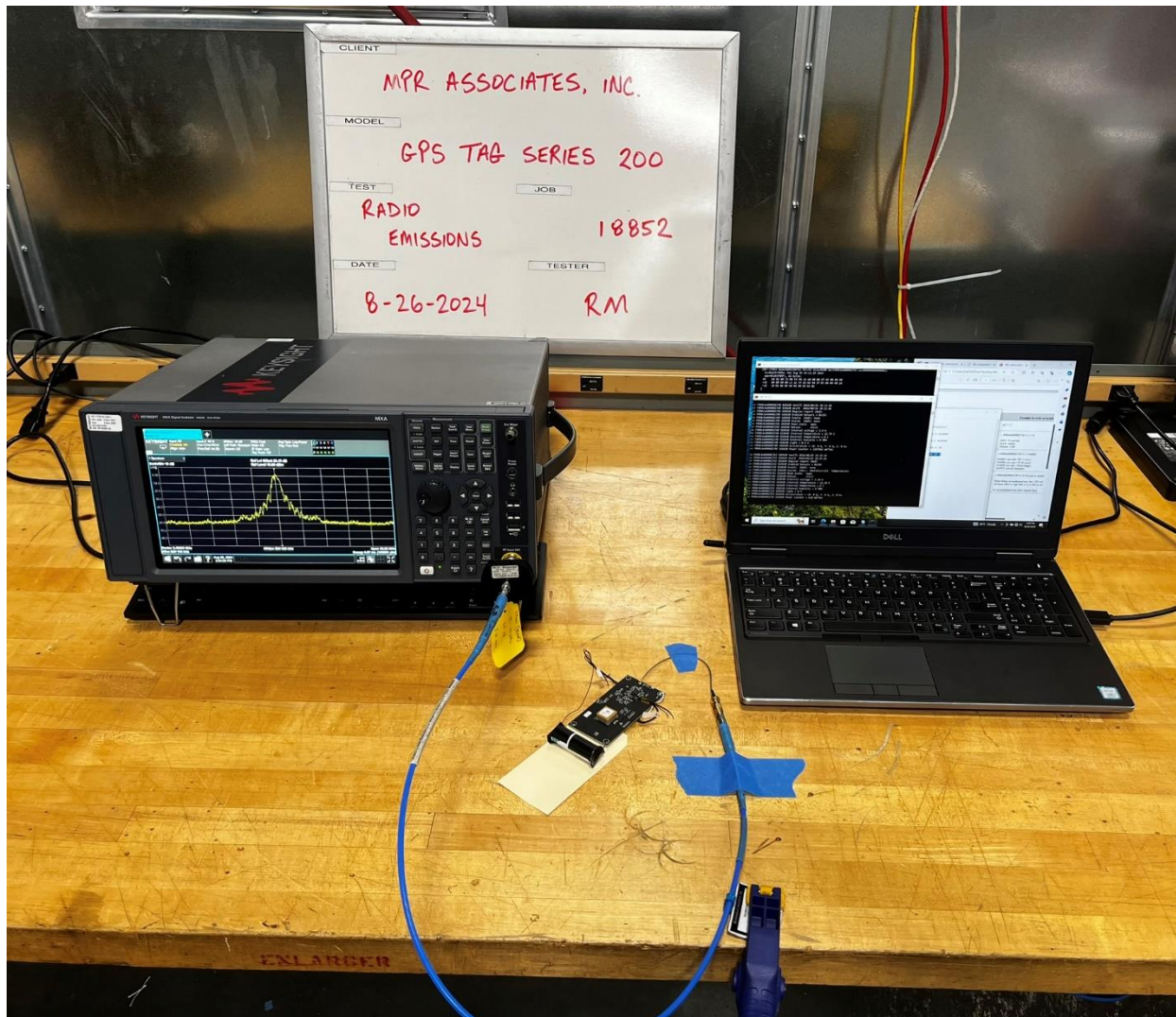
Conducted Radio Emissions View 1
