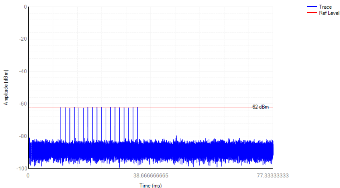
Radar Calibration
