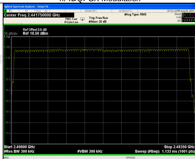
8DPSK Modulation
