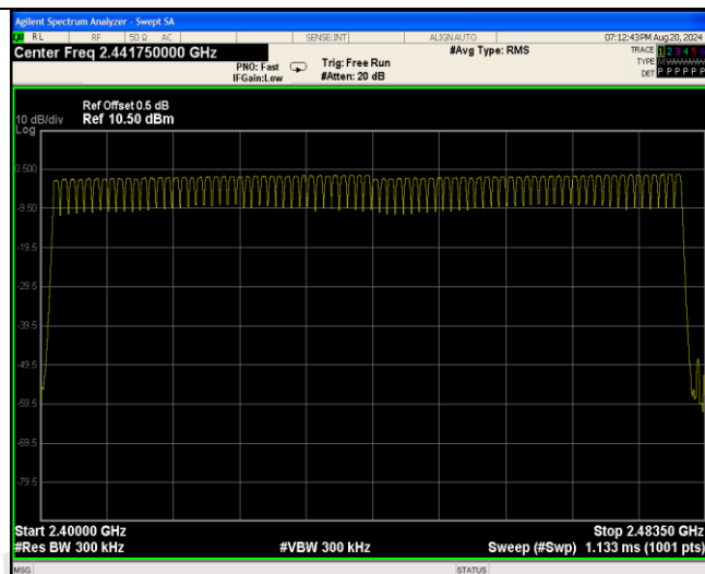
GFSK Modulation
