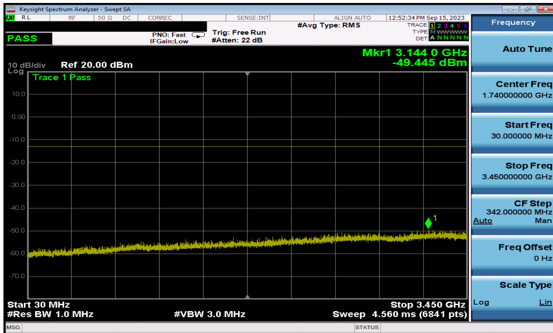
Plot 7-38. Conducted Spurious Plot (NR Band n78 - 10MHz QPSK - High Channel)
