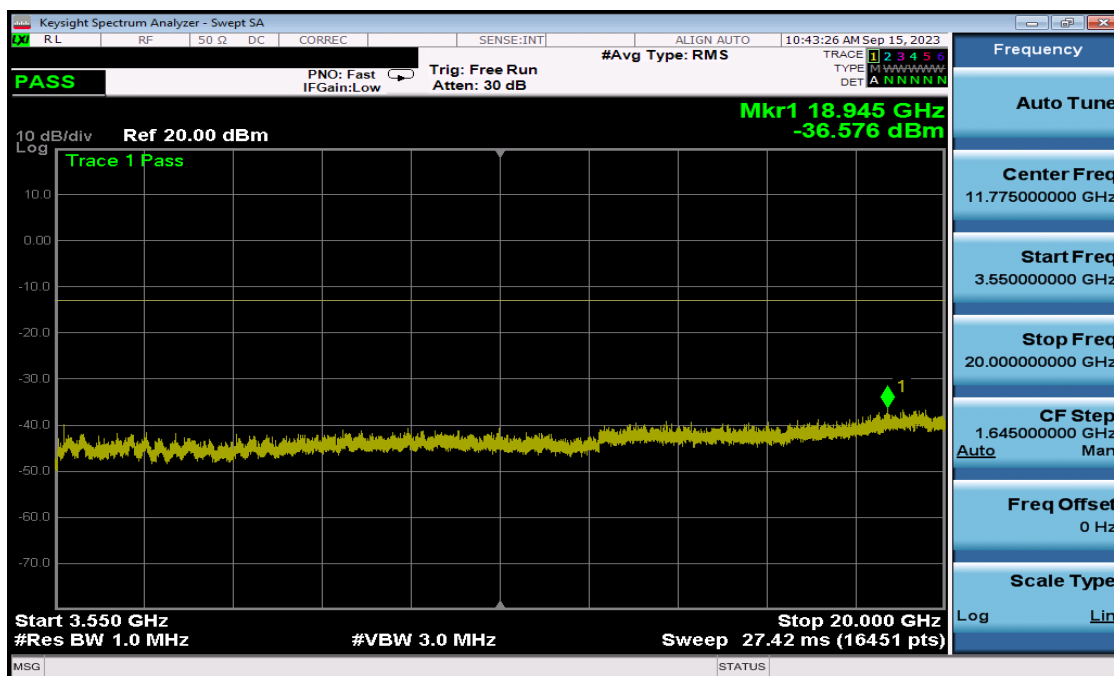
Plot 7-15. Conducted Spurious Plot (NR Band n78 - 10MHz QPSK - Mid Channel)
