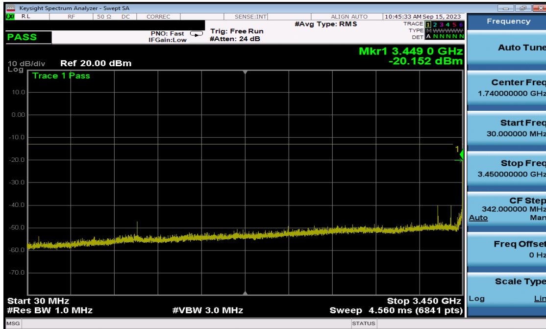
Plot 7-11. Conducted Spurious Plot (NR Band n78 - 10MHz QPSK - Low Channel)
