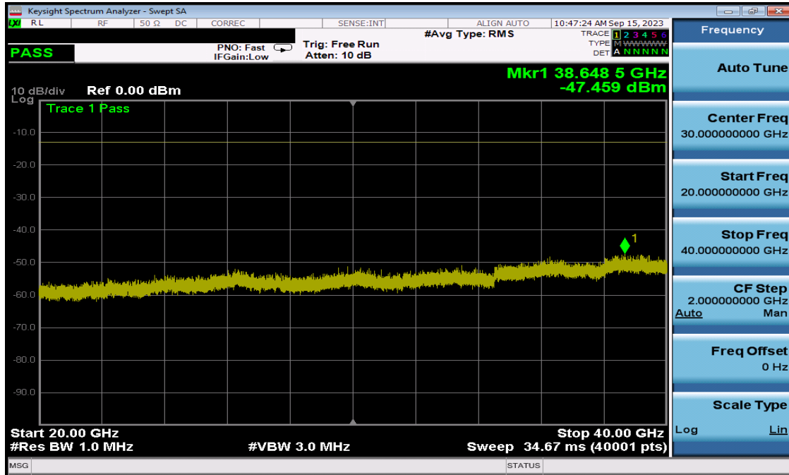
Plot 7-13. Conducted Spurious Plot (NR Band n78 - 10MHz QPSK - Low Channel)
