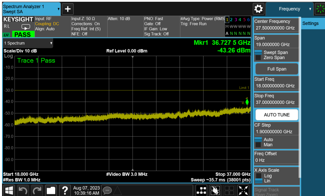
Plot 7-37. Conducted Spurious Plot (NR Band n78 - 10MHz QPSK - Low Channel)
