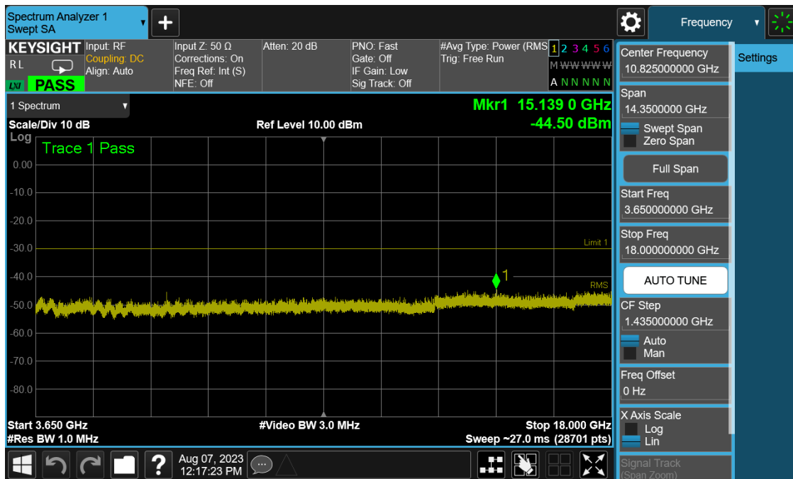
Plot 7-30. Conducted Spurious Plot (NR Band n78 - 10MHz QPSK - Low Channel)
