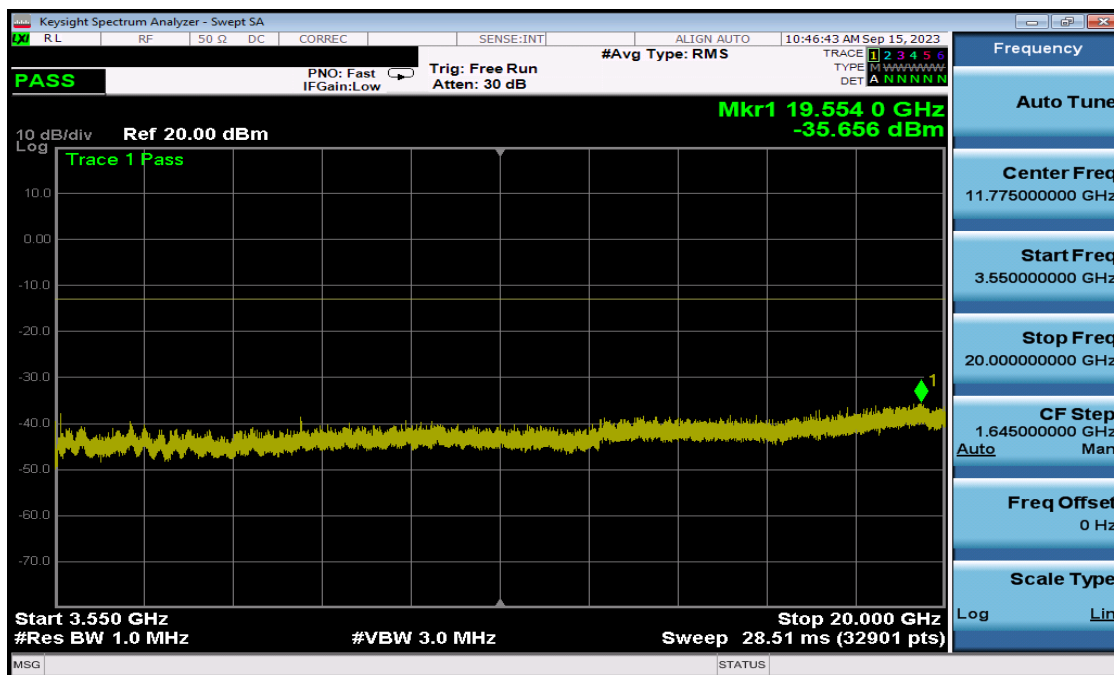
Plot 7-12. Conducted Spurious Plot (NR Band n78 - 10MHz QPSK - Low Channel)
