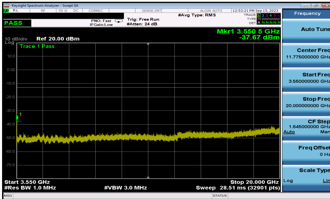
Plot 7-39. Conducted Spurious Plot (NR Band n78 - 10MHz QPSK - High Channel)
