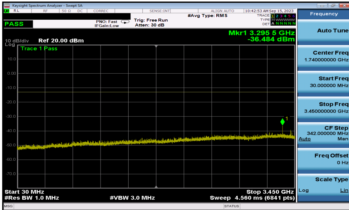
Plot 7-14. Conducted Spurious Plot (NR Band n78 - 10MHz QPSK - Mid Channel)
