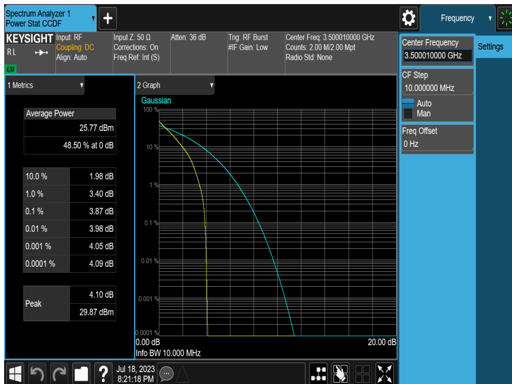
Plot 7-49.PAR Plot (NR Band n78 - 10MHz DFT-s-OFDM BPSK– Full RB)
