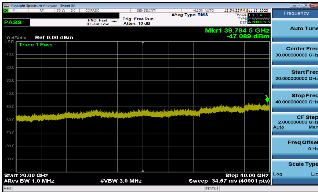
Plot 7-40. Conducted Spurious Plot (NR Band n78 - 10MHz QPSK - High Channel)
