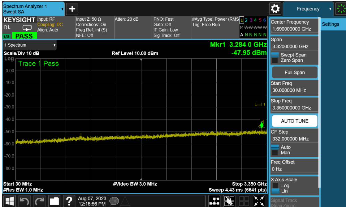
Plot 7-29. Conducted Spurious Plot (NR Band n78 - 10MHz QPSK - Low Channel)
