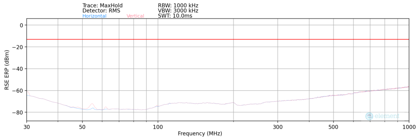
Plot 7-63. Radiated Spurious Plot Below 1GHz (UL-MIMO NR Band 78)
