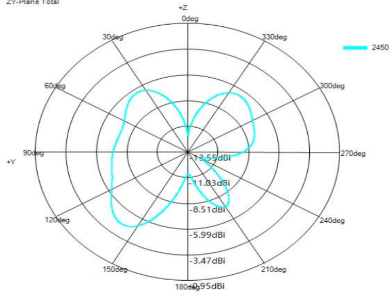
ZY-Plane Total
