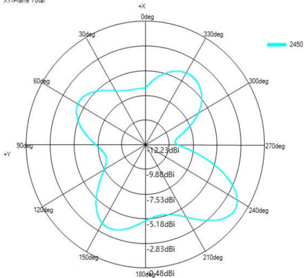
XY-Plane Total
