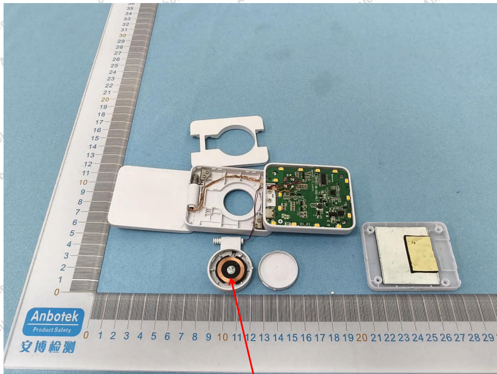
Watch-ANT
