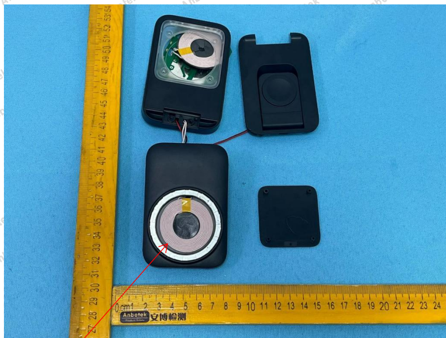
Phone ANT
