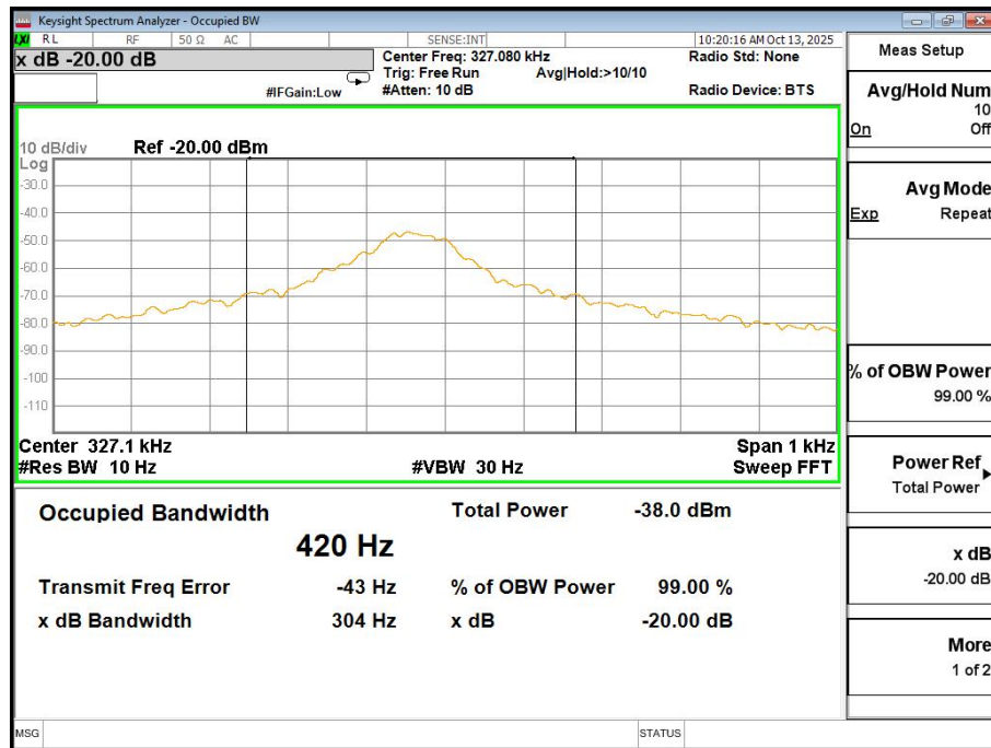
iWatch coil
