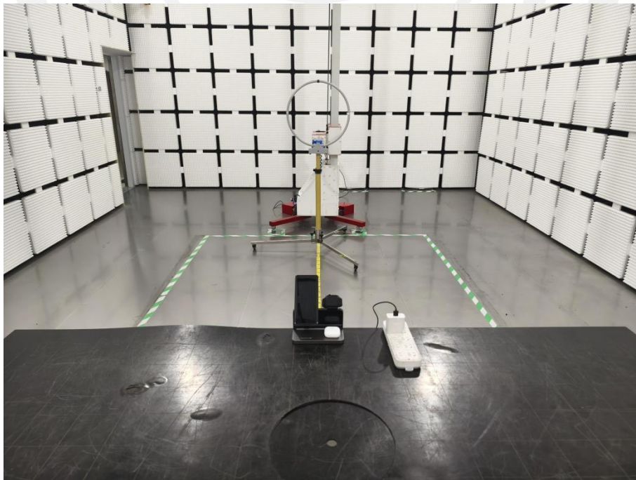
Spurious Radiation Emissions Test (<30MHz)
