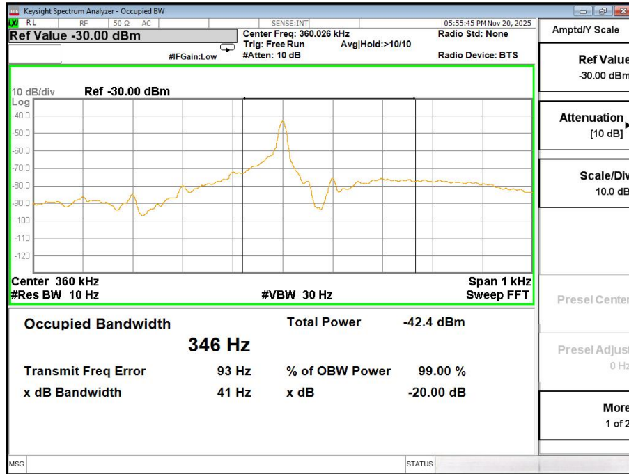
Phone coil (360KHz)
