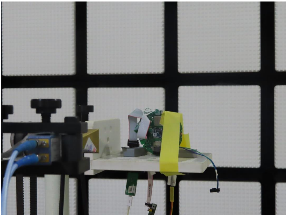
50GHz ~ 75GHz
