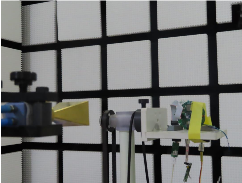
50GHz ~ 75GHz
