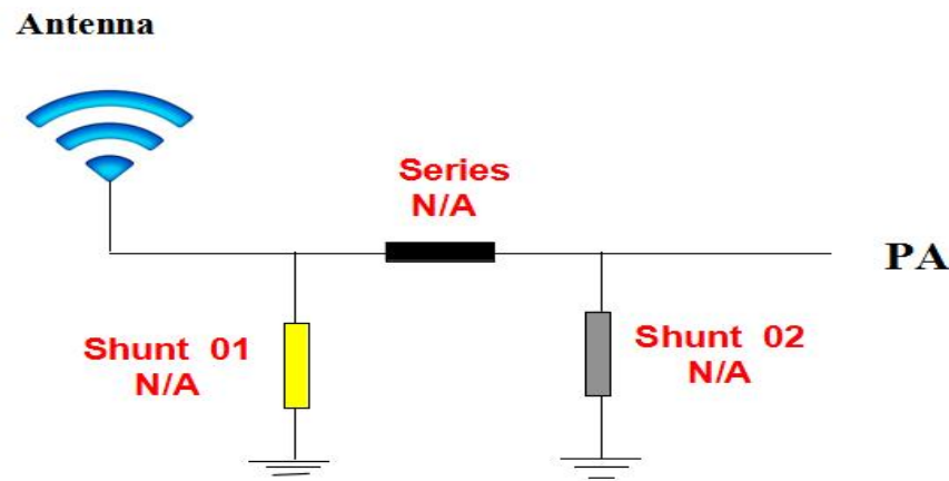
1-3 Impedance matching
