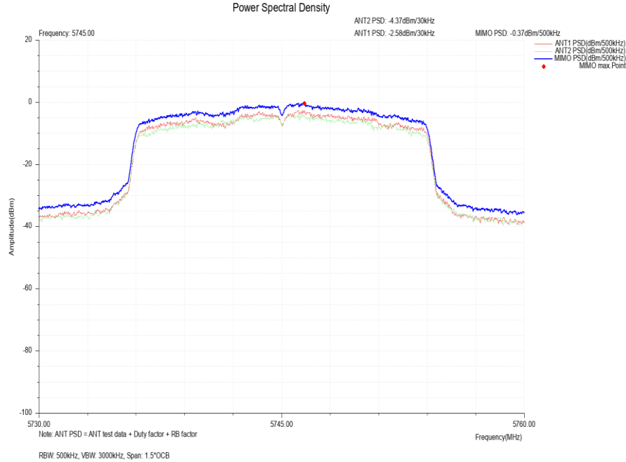
NVNT_MIMO_TX_802_11n(HT20)_Power_Spectral_Density_5745
