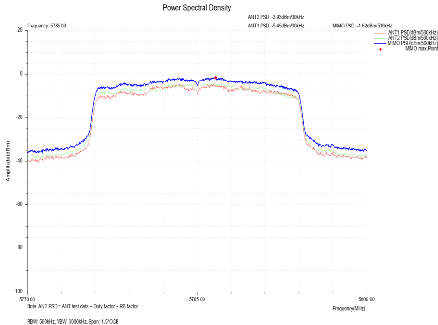
NVNT_MIMO_TX_802_11n(HT20)_Power_Spectral_Density_5785
