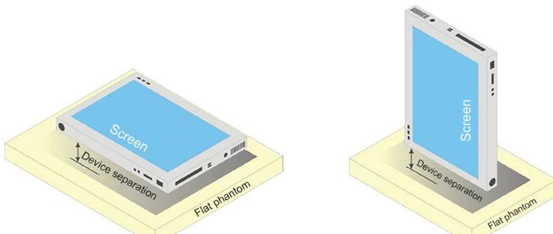
F-11. Test positions for body-worn devices
