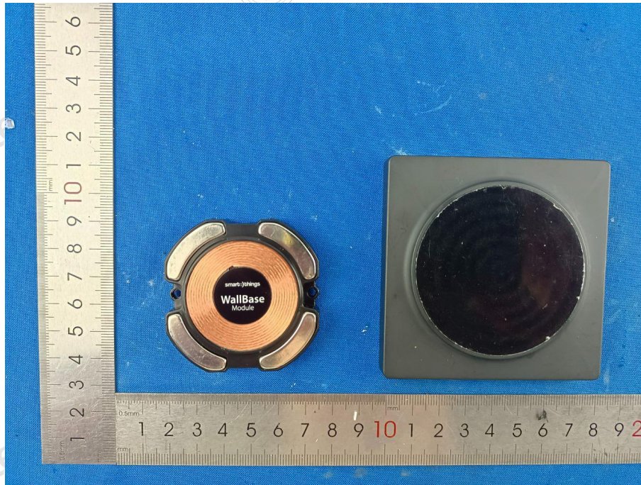
Hardware version: Small-sized housing EUT: WB-Module-0100
