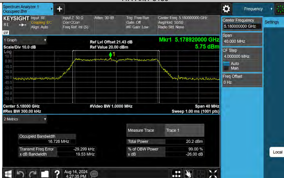
11A-Ant2-5180
