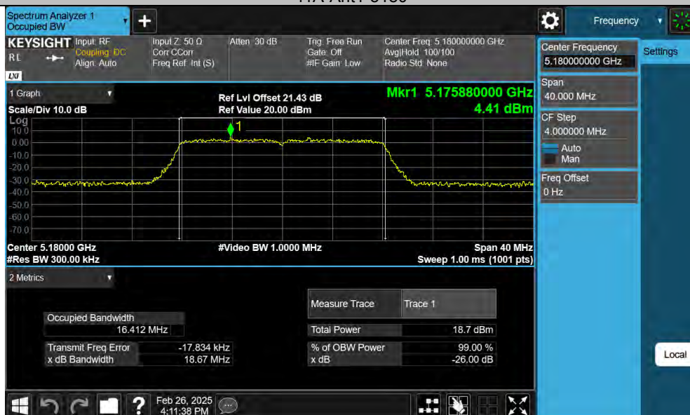
11A-Ant2-5180
