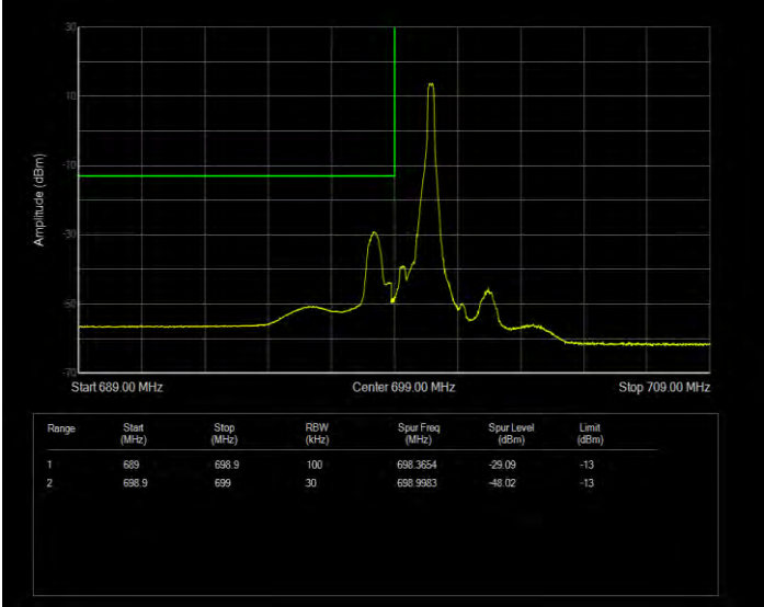
Band12 16QAM BW=1.4MHz Channel=23017 RB Size=6 Position=#0 Extended
