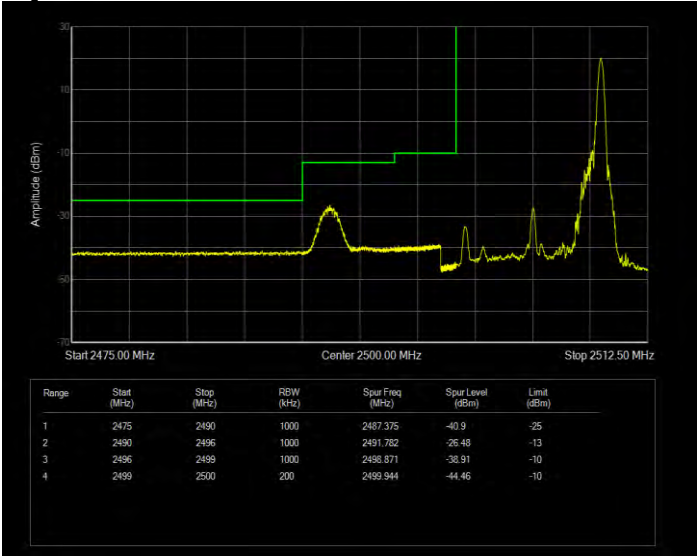
Band7 16QAM BW=10MHz Channel=20800 RB Size=50 Position=#0 Extended
