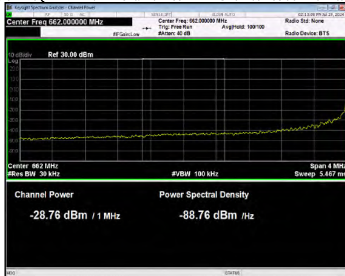
Band71 16QAM BW=20MHz Channel=133222 RB Size=100 Position=#0 Extended
