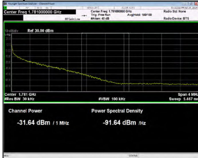
Band66 16QAM BW=20MHz Channel=132572 RB Size=1 Position=#Max Normal
