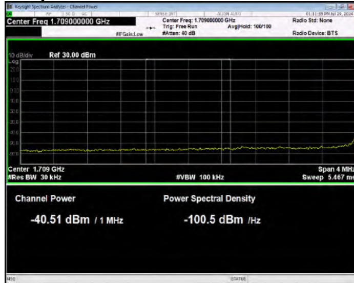
Band66 16QAM BW=20MHz Channel=132072 RB Size=1 Position=#Max Normal
