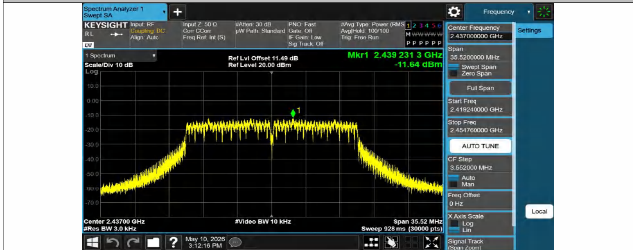
11N20SISO-Ant1-2437-PASS
