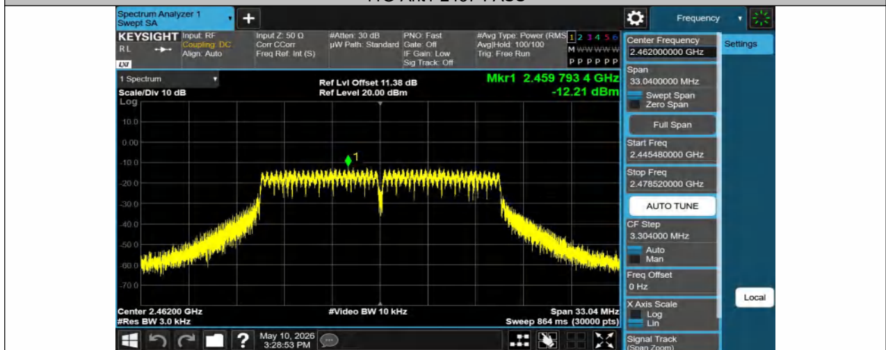
11G-Ant1-2462-PASS
