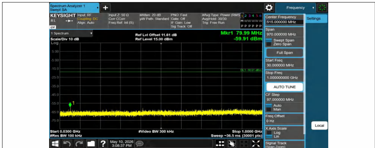
11N20SISO-Ant1-2412-30~1000-PASS
