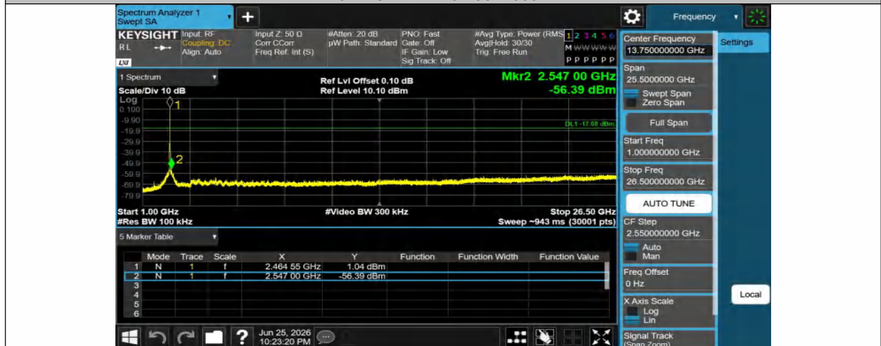
11N20SISO-Ant1-2462-1000~26500-PASS
