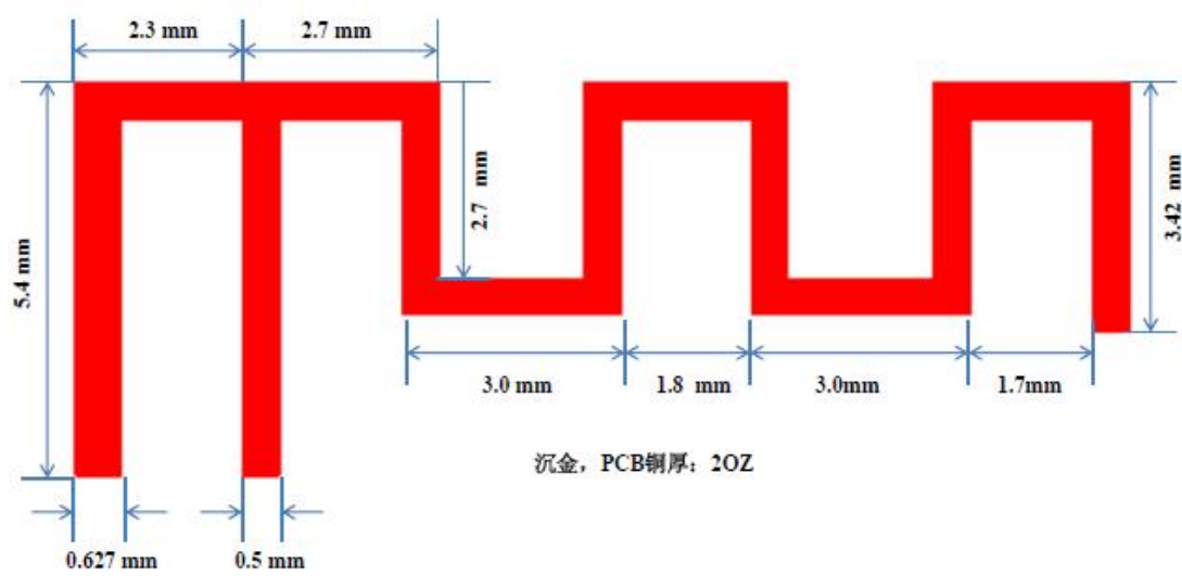
Antenna Dimension
