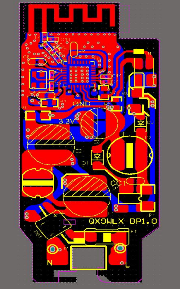
CX011-on-board-antenna
