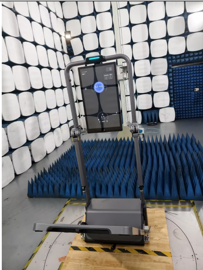
Radiated Spurious Emission, Above 1GHz
