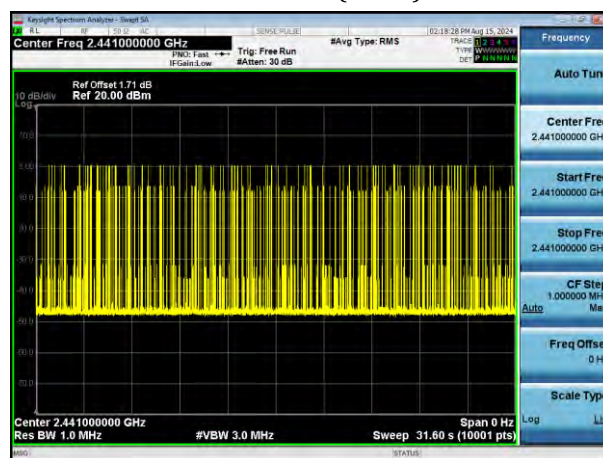
Accumulate(3DH5)
