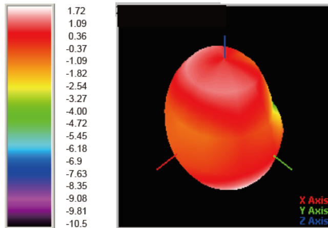
© 3D Gain Pattern (2450 MHz) Unit:dBi
