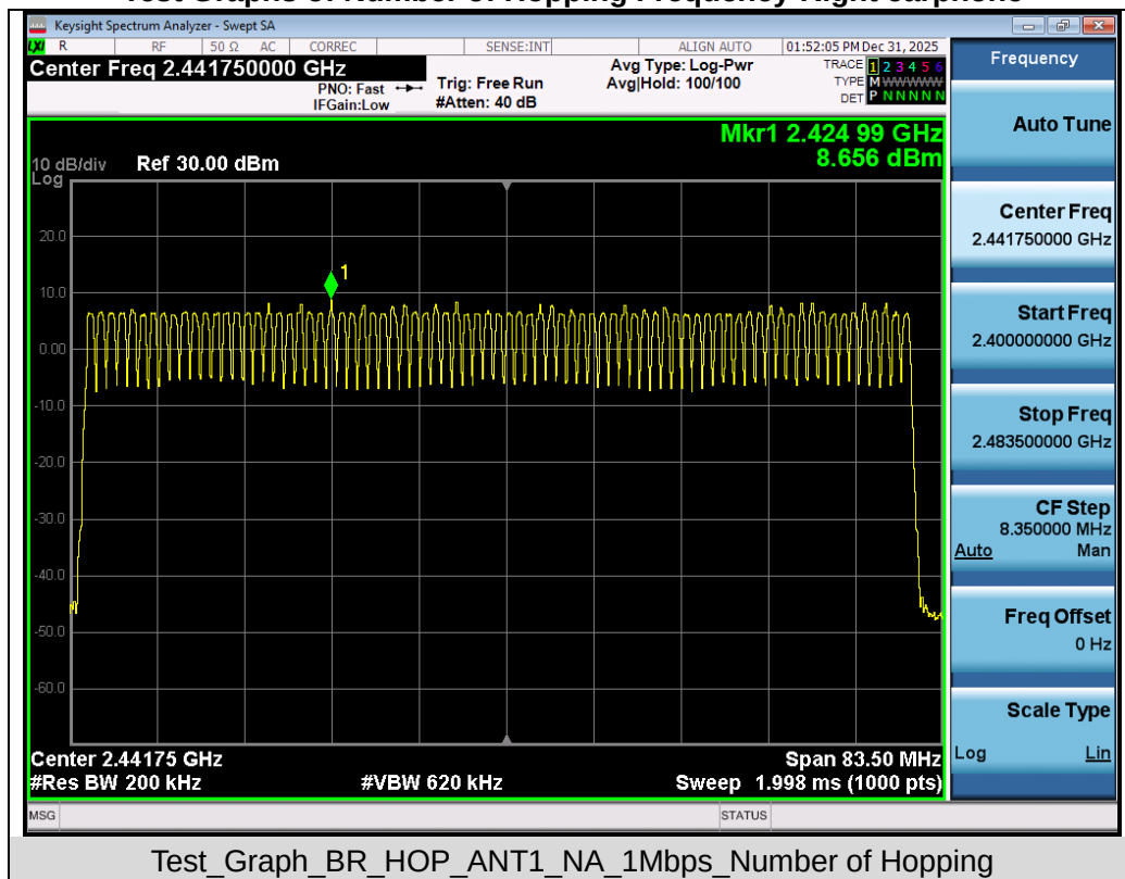
Test Graphs of Number of Hopping Frequency-Right earphone
