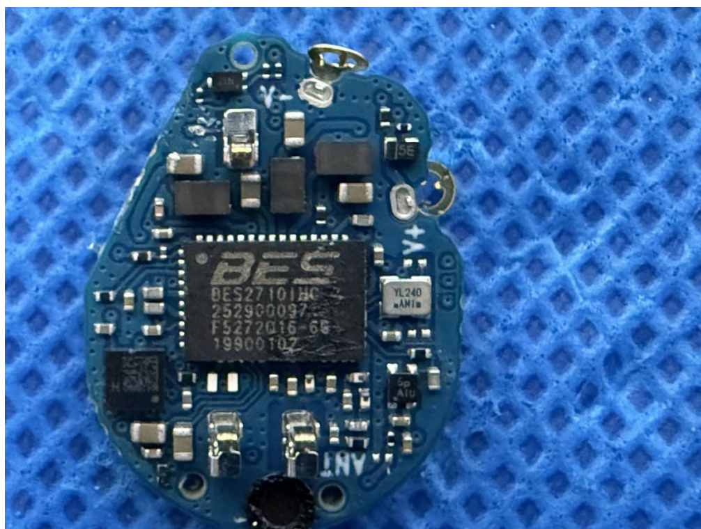
Internal view-3 of EUT(Left Ear)
