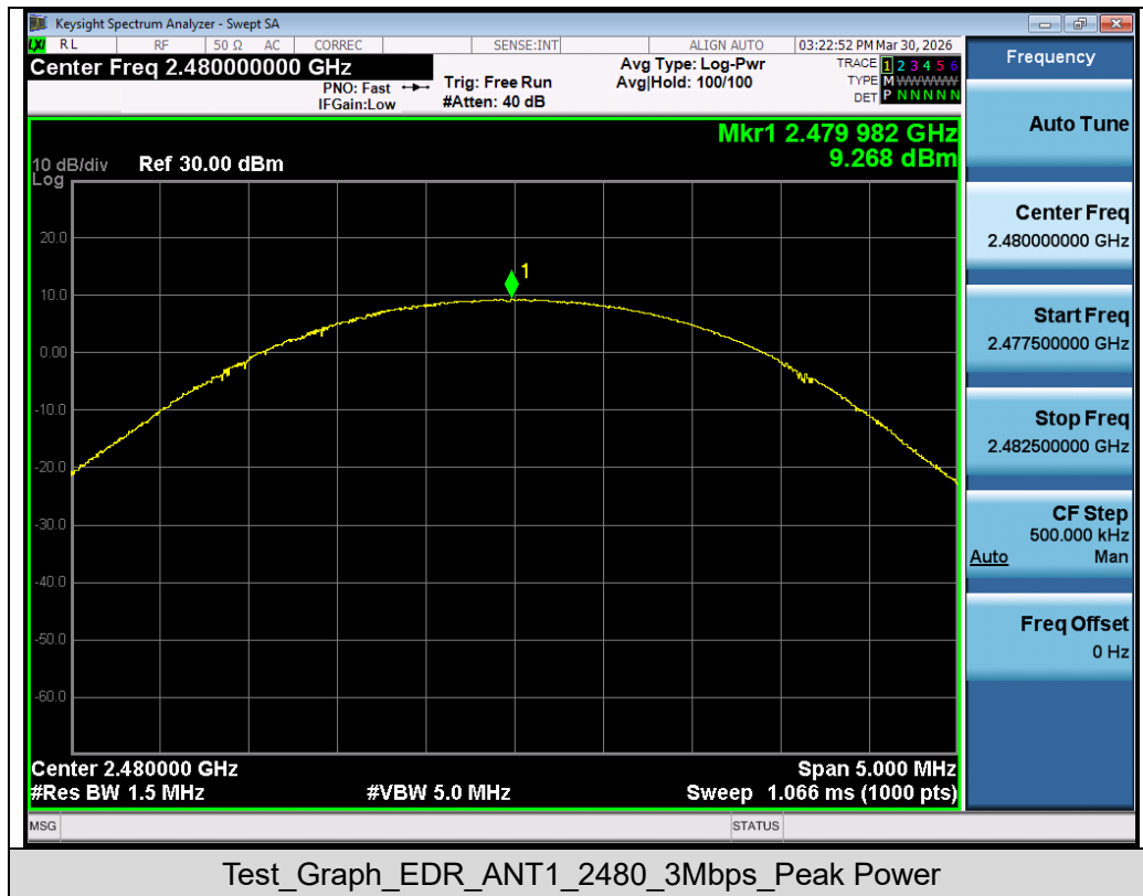
Test Graphs of Conducted Output Power-Right earphone
