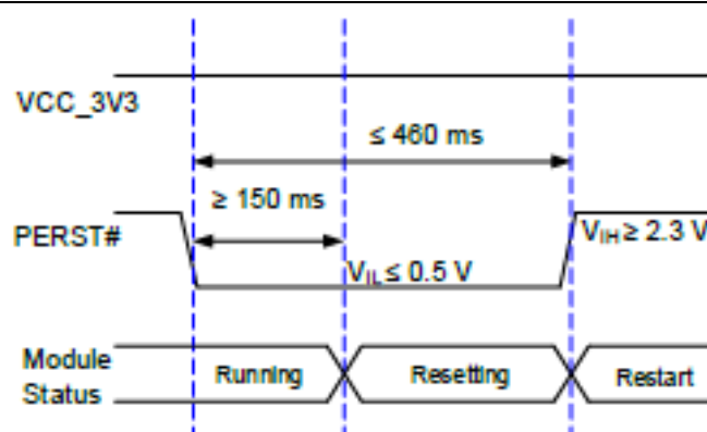
Figure 12: Reset Timing
