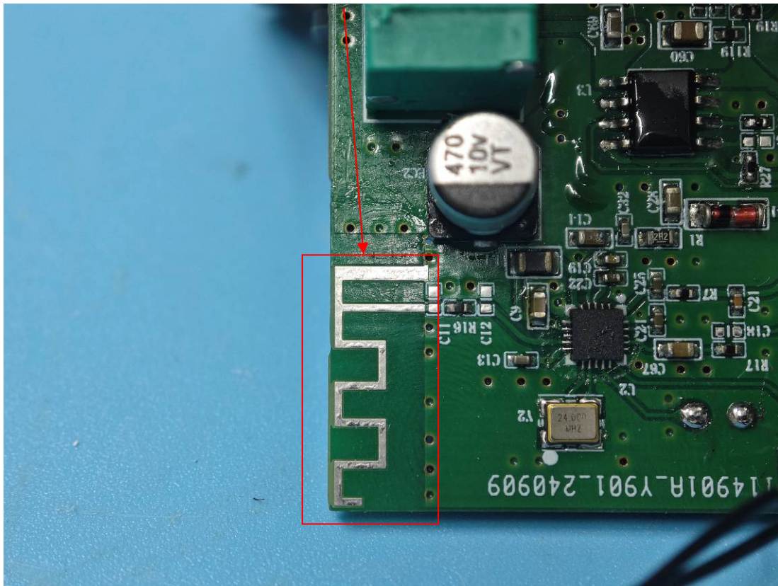
BT Antenna-Only Receiver
