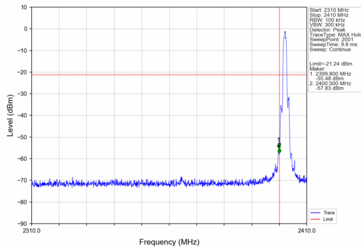
Pi/4DQPSK_2DH5_LCH_2402MHz_Ant1_NTNV
