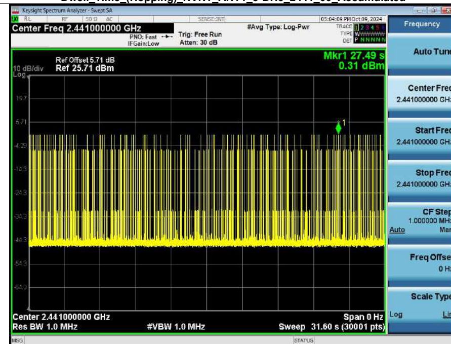
Dwell_Time (Hopping)_NVNT_ANT1_3-DH5_2441_00_Accumulated
