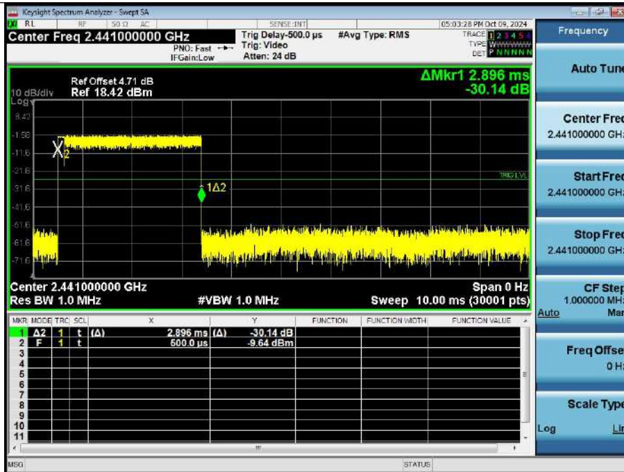
Dwell_Time (Hopping)_NVNT_ANT1_3-DH5_2441_00_Accumulated
