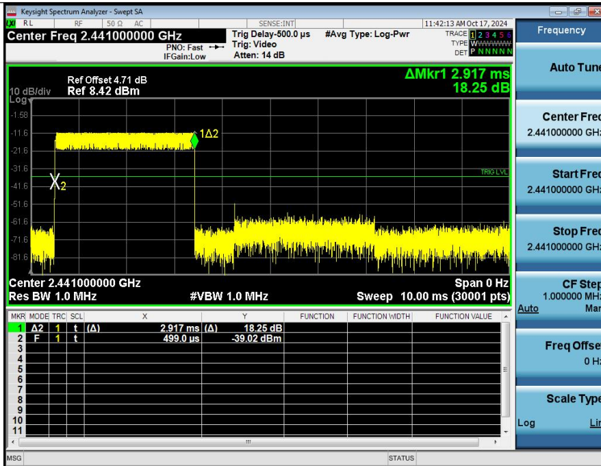
Dwell Time (Hopping) HVNT_ANT1_1-DH5_2441_00_Accumulated
