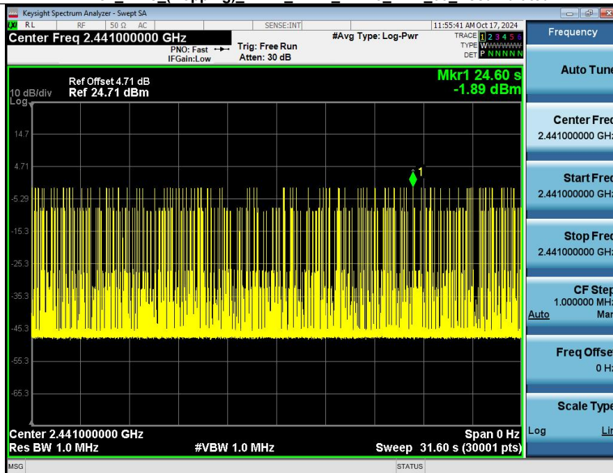
Dwell Time (Hopping) HVNT_ANT1_2-DH5_2441_00_Accumulated
