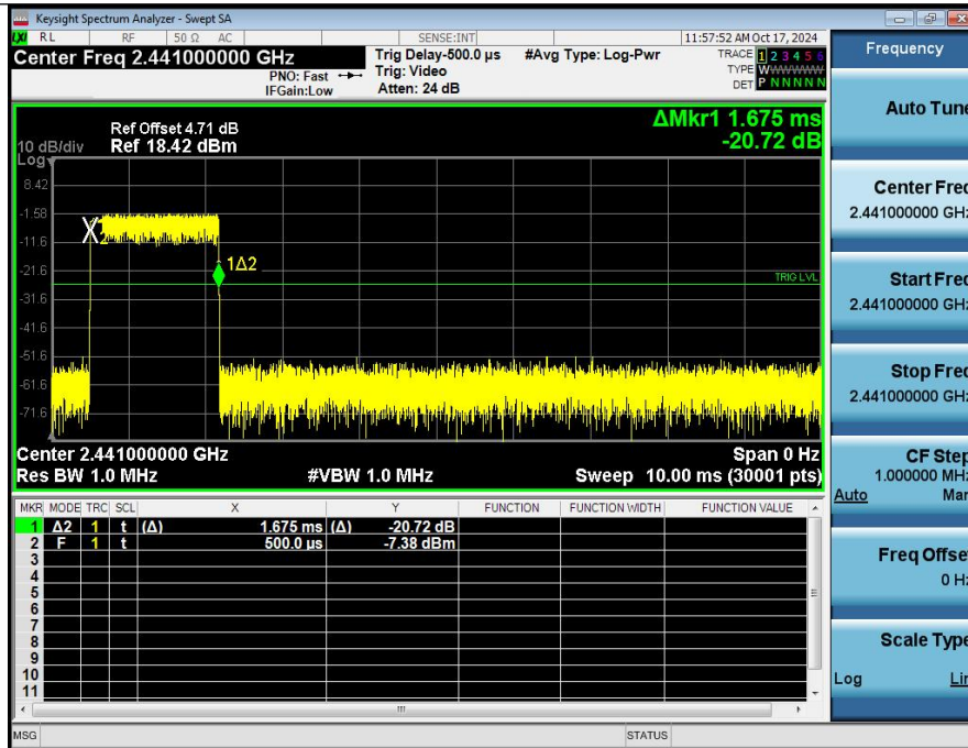
Dwell Time (Hopping) HVNT_ANT1_3-DH3_2441_00_Accumulated
