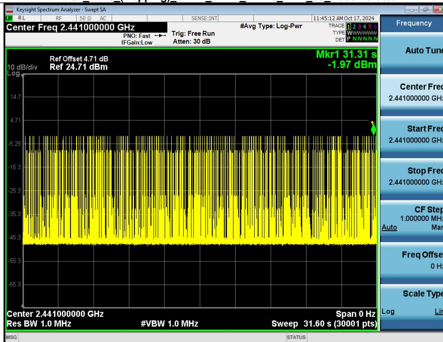
Dwell Time (Hopping) HVNT_ANT1_2-DH3_2441_00_Accumulated
