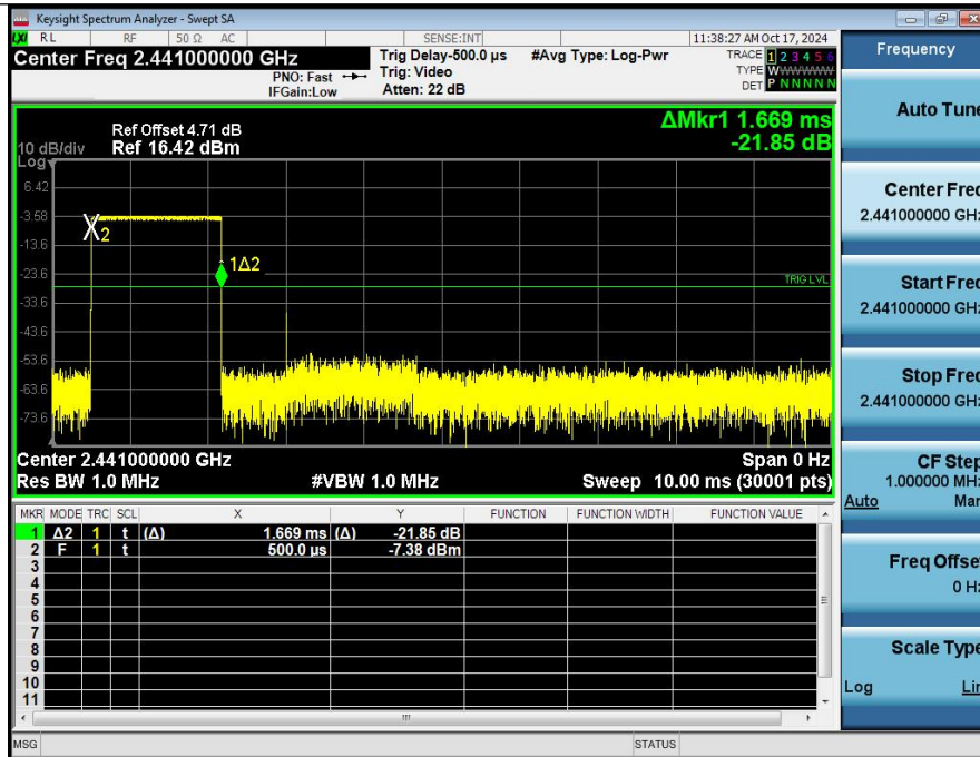
Dwell Time (Hopping) HVNT_ANT1_1-DH3_2441_00_Accumulated
