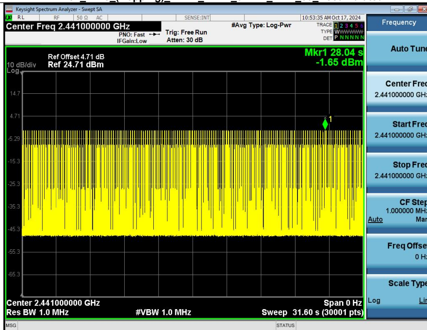
Dwell Time (Hopping) HVNT_ANT1_3-DH1_2441_00_Accumulated
