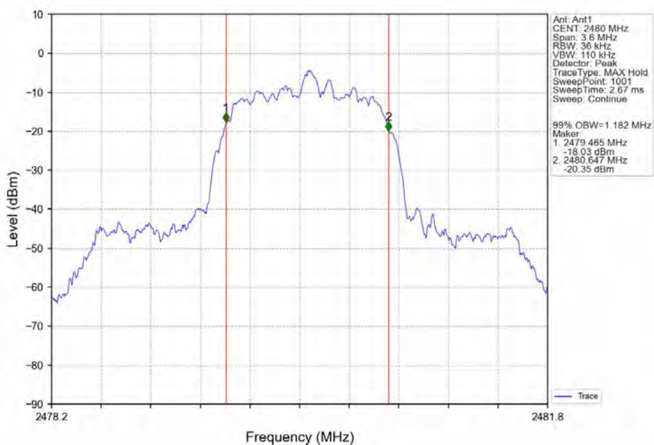
\pi/4 DQPSKK_2DH5_HCH_2480MHz_Ant1_NTNV
