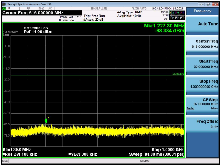
2DH5-Ant1-2480-30~1000-PASS
