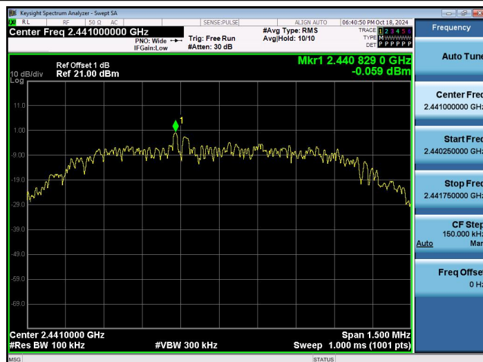
2DH5-Ant1-2441-0~Reference-PASS
