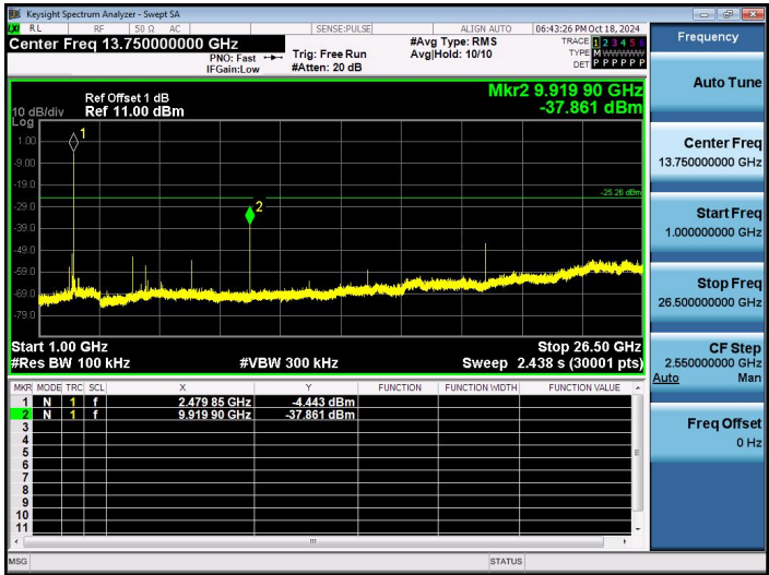
2DH5-Ant1-2480-1000~26500-PASS
