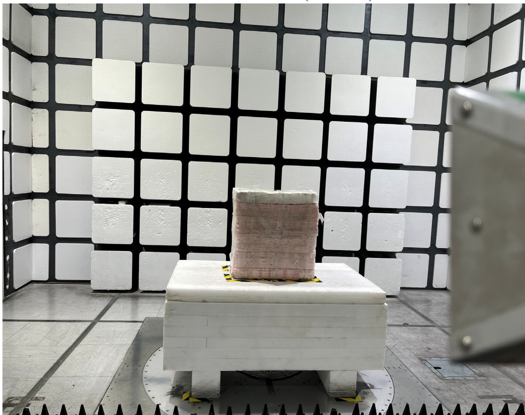
Radiated Emissions View (18-25 GHz)
