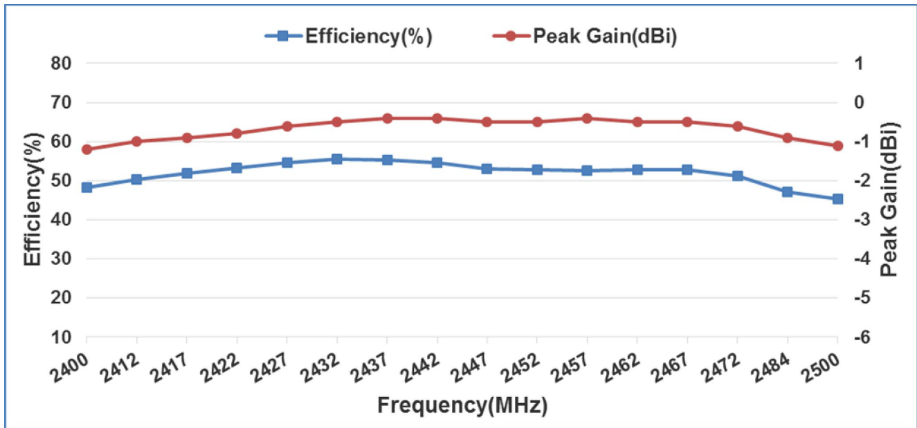
6-4-2-3. 3D Efficiency vs. Frequency
