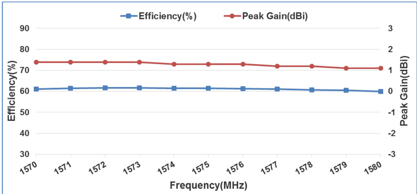
5-4-1-3. 3D Efficiency vs. Frequency
