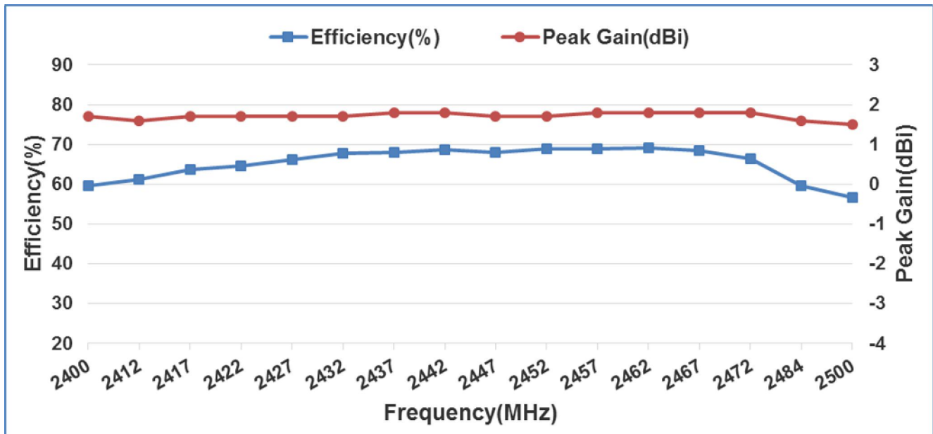
5-4-2-3. 3D Efficiency vs. Frequency
