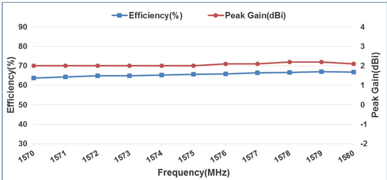
6-4-1-3. 3D Efficiency vs. Frequency
