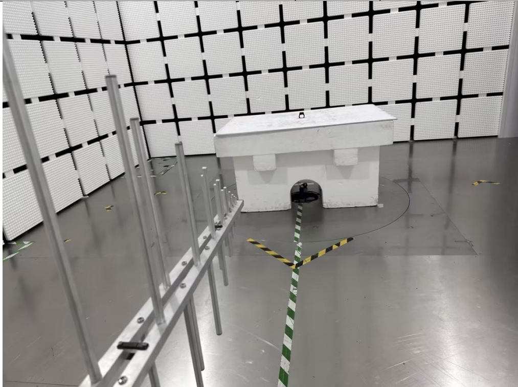
Radiated Emission Above 1G (SRD 2405M)
