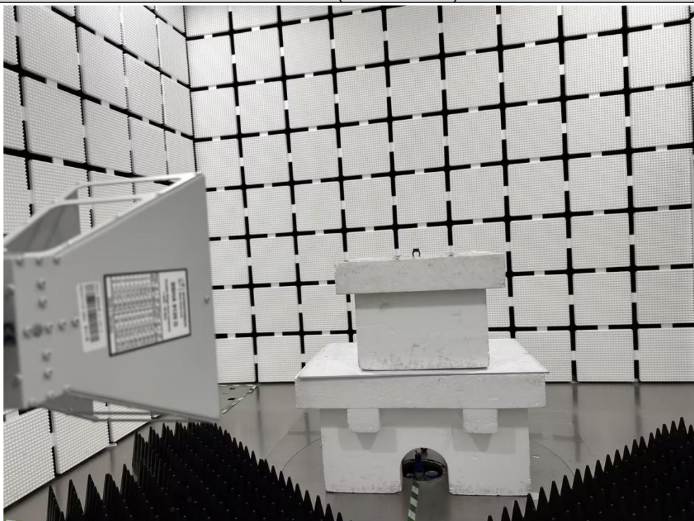
Conducted test (SRD 2405M)
