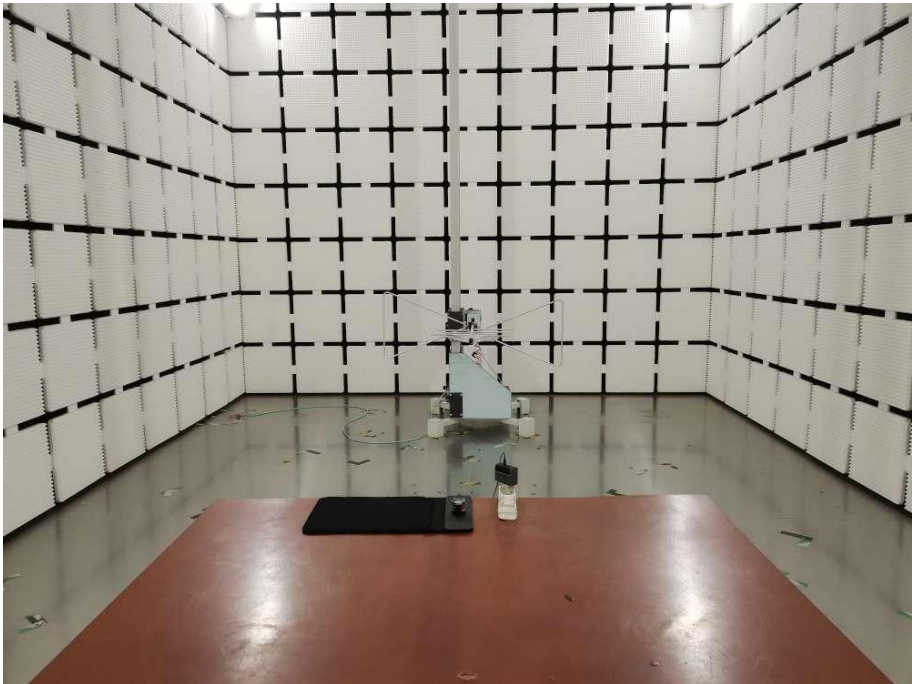
Radiated Emission Test View 5
