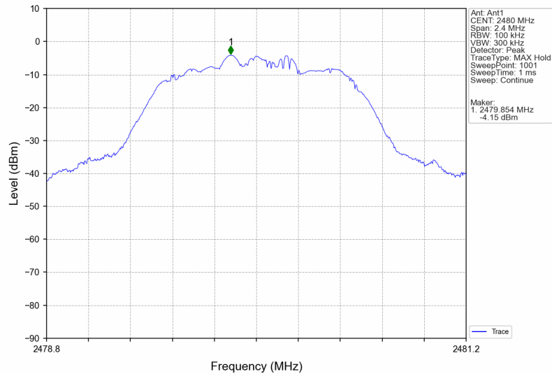
8DPSK_3DH5_HCH_2480MHz_Ant1_NTNV
