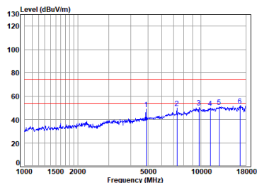
BT_3DH5_TX_CH_39_Horizontal
