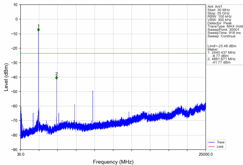
Pi/4DQPSK_2DH5_MCH_2441MHz_Ant1_NTNV
