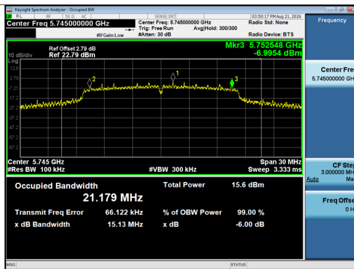
-6dB Bandwidth NVNT 5745MHz Ant1
